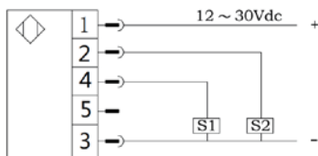
2 × PNP
