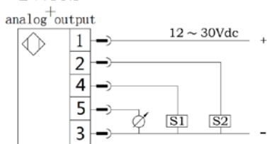
2 × PNP
